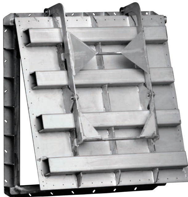
RC Square Flap Gate
