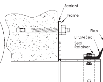
Detail view of Section A-A
