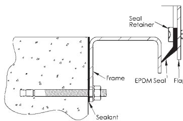
Detail view of Section C-C
